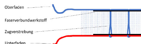
Fig. 3: Double lockstitch for sewing fiber composite tanks
